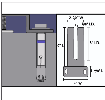
Seismic approved drop-in concrete anchor
