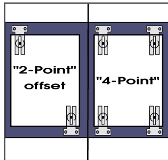
Fastening Methods
