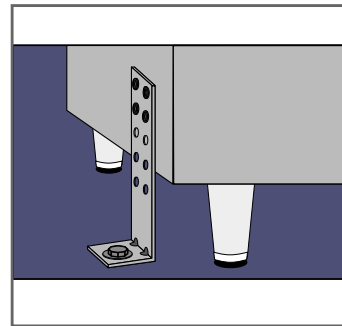
"2-point" offset or "4-point" floor fastening
