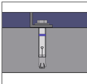
Floor kit comes with seismic rated concrete anchors
