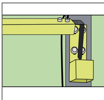
Close up of shoe bracket and drop pin
